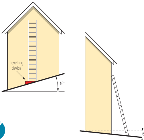
Figure 3 Ladder showing maximum angles at 16° on a side slope and 6° on a back slope
